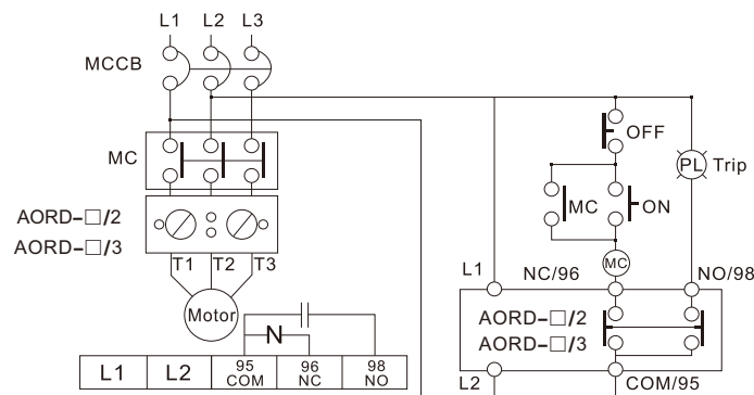
Description diagram for AORD-□/2, AORD-□/3
